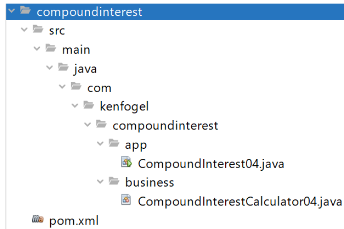
Figure 3.4 – Basic Maven file structure
