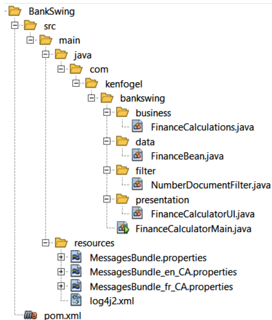
Figure 13.5 – The Swing project layout
