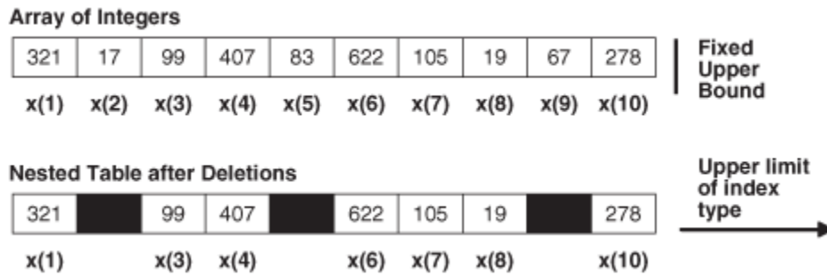
Figure 5-2 Array and Nested Table
